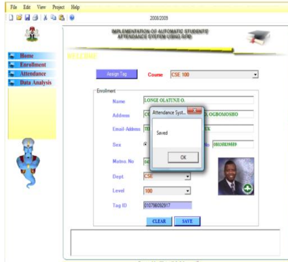
Fig. 6. Enrolment Interface
